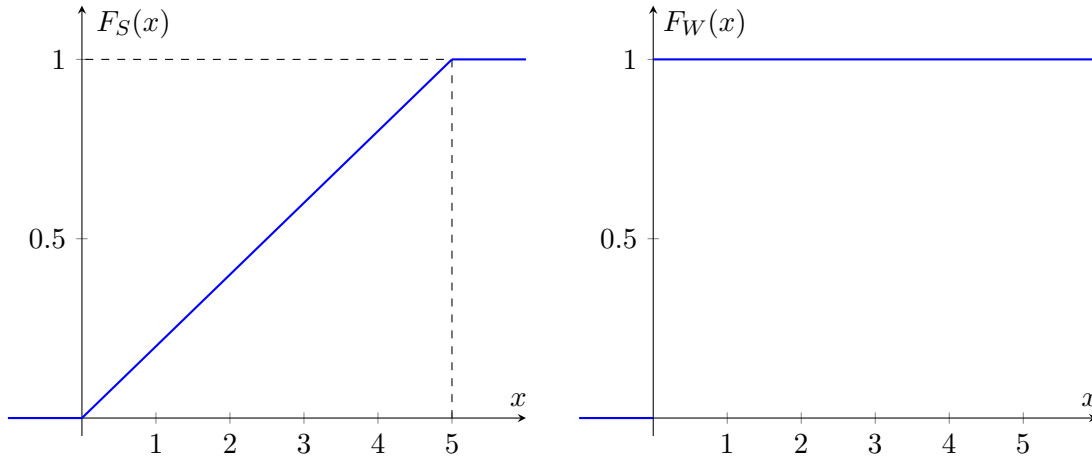
Figure 1: The distributions of the S - and W -type players, in equilibrium, given s_1 = 10 , s_2 = 5 , w_1 = 4 , and w_2 = 2 (these values meet the conditions of Proposition ??).
