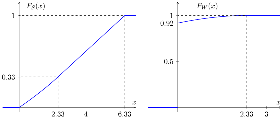
Figure 3: The distributions of the S - and W -type players, in equilibrium, given s_1 = 10, s_2 = 4, w_1 = 5 , and w_2 = 4 . These values meet the conditions of Proposition ??.
