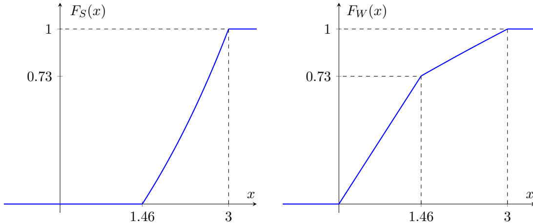
Figure 5: The distributions of the S - and W -type players, in equilibrium, given s_1 = 5 , s_2 = 2 , w_1 = 3 , and w_2 = 2 . These values sustain the conditions of Proposition ??.
