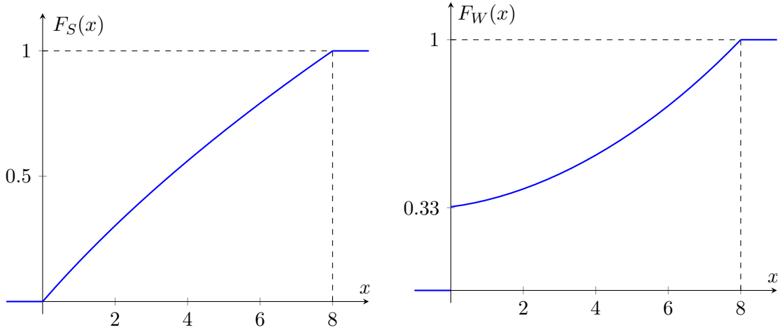
Figure 2: The distributions of the S - and W -type players, in equilibrium, given s_1 = 10, s_2 = 6, w_1 = 8 , and w_2 = 3 . Note that these parameters meet the conditions of Proposition ??.
