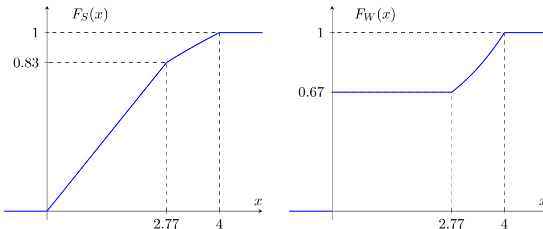
Figure 6: The distributions of the S - and W -type players, in equilibrium, given s_1 = 8, s_2 = 6, w_1 = 4 , and w_2 = 0 (as given in Claim ??).
